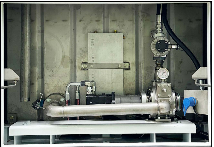
Passenger Side DEF Pump Cabinet
