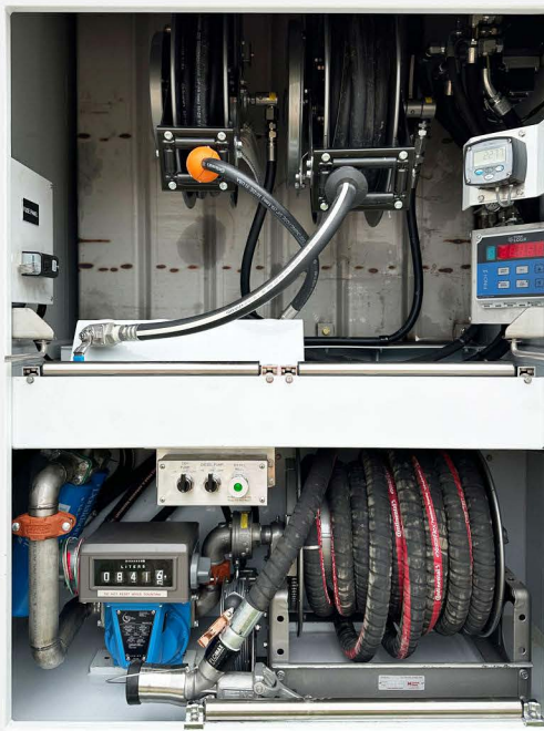
Drivers Side Dispense Cabinet
